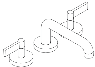
ONE DECK-MOUNT BATH SET, LOW SPOUT, LEVER HANDLES P24404-LV HEIGHT: 4½" SPREAD: 8" REACH: 7" REQUIRED ¾" CERAMIC HIGH-FLOW VALVE SYSTEM: P19302
