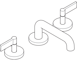
ONE BASIN SET, LOW SPOUT, LEVER HANDLES P24401-LV HEIGHT: 3" SPREAD: 8" REACH: 5½"
