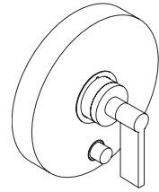
ONE PRESSURE BALANCE VALVE WITH DIVERTER, LEVER HANDLE P24416-LV DIAMETER: 6 1 / 4 " REQUIRED ROUGH-IN: P19300
