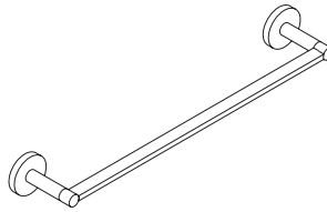
ONE TOWEL BAR, 18" P34402-00 WIDTH: 20 1 / 4 " HEIGHT: 2 1 / 4 " DEPTH: 3 1 / 2 "
