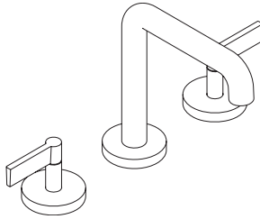
ONE BASIN SET, TALL-SPOUT, LEVER HANDLES P24402-LV HEIGHT: 6½" SPREAD: 8" REACH: 5½"
