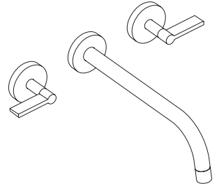
ONE WALL-MOUNT BASIN SET, LEVER HANDLES P24411-LV SPREAD: 9" SPOUT REACH: 10½" REQUIRED ROUGH-IN: P29304-00
