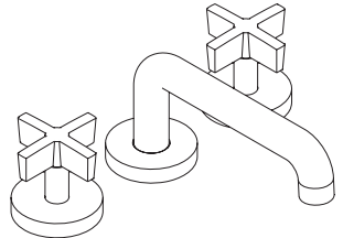
ONE DECK-MOUNT BATH SET, LOW SPOUT, CROSS HANDLES P24404-CR HEIGHT: 4½" SPREAD: 8" REACH: 7" REQUIRED ¾" CERAMIC HIGH-FLOW VALVE SYSTEM: P19302
