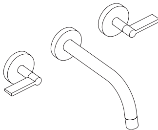
ONE WALL-MOUNT BASIN SET, LEVER HANDLES P24410-LV SPREAD: 9" SPOUT REACH: 7½" REQUIRED ROUGH-IN: P29304-00
