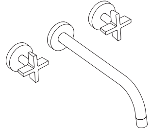
ONE WALL-MOUNT BASIN SET, CROSS HANDLES P24411-CR SPREAD: 9" SPOUT REACH: 10½" REQUIRED ROUGH-IN: P29304-00
