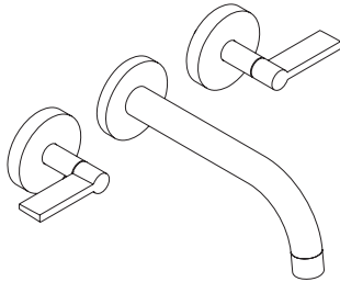
ONE WALL-MOUNT BATH SET WITH SPOUT, LEVER HANDLES P24425-LV SPREAD: 8" SPOUT REACH: 8 1 / 16 " REQUIRED ROUGH-IN: P29517-00
