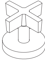
ONE DECK DIVERTER, CROSS P24420-CR WIDTH: 3" HEIGHT: 2 7 / 8 " REQUIRED DECK DIVERTER VALVE: P29515
