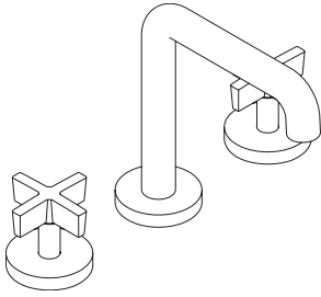
ONE DECK-MOUNT BATH SET, TALL-SPOUT, CROSS HANDLES P24405-CR HEIGHT: 8 13 / 16 " SPREAD: 8" REACH: 7 3 / 16 " REQUIRED 3 / 4 " CERAMIC HIGH-FLOW VALVE SYSTEM: P19302
