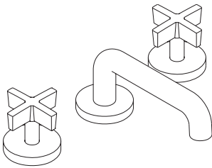
ONE BASIN SET, LOW SPOUT, CROSS HANDLES P24401-CR HEIGHT: 3" SPREAD: 8" REACH: 5½"
