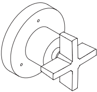
ONE 3-WAY TRANSFER VALVE TRIM, CROSS HANDLE P24483-CR DIAMETER: 3¾" REQUIRED ROUGH-IN: P29513
