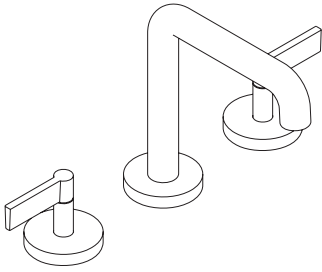
ONE DECK-MOUNT BATH SET, TALL-SPOUT, LEVER HANDLES P24405-LV HEIGHT: 8 13 / 16 " SPREAD: 8" REACH: 7 3 / 16 " REQUIRED 3 / 4 " CERAMIC HIGH-FLOW VALVE SYSTEM: P19302
