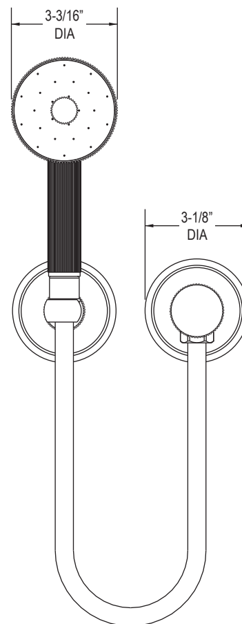
Rough-In Information
