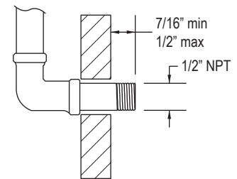
Rough-In Information
