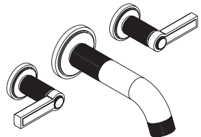
VIR STIL WALL-MOUNT BATH SET WITH LEVER HANDLES P24125-LV REACH: 7" REQUIRED (ONE OF EACH): ROUGH-IN, HOT P29504-XX ROUGH-IN, COLD P29504-XY
