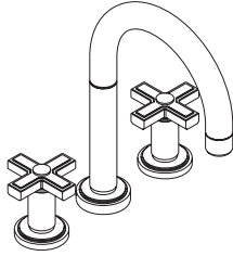
VIR STIL MINIMAL DECK-MOUNT BATH SET WITH CROSS HANDLES P24104-CR REQUIRED: ¾" CERAMIC HIGH-FLOW VALVE SYSTEM P19302-00 HEIGHT: 12¾" SPREAD: 8" REACH: 7¾"
