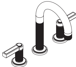
VIR STIL DECK-MOUNT BATH SET WITH LEVER HANDLES P24103-LV REQUIRED: ¾" CERAMIC HIGH-FLOW VALVE SYSTEM P19302-00 HEIGHT: 12¾" SPREAD: 8" REACH: 7½"
