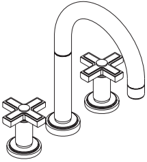
VIR STIL MINIMAL BASIN SET WITH CROSS HANDLES P24101-CR HEIGHT: 9½" SPREAD: 8" REACH: 5¾"
