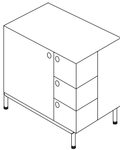
VIR STIL VANITY IN WHITE LACQUER P74201-WH REQUIRED ACCESSORY: METAL VANITY BASE & COORDINATING DRAWER AND DOOR PULLS P74202-LG WIDTH: 32 1 / 2 " HEIGHT: 33 1 / 2 " DEPTH: 22" (WITH TOP AND LEGS)
