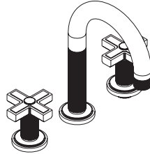
VIR STIL DECK-MOUNT BATH SET WITH CROSS HANDLES P24103-CR REQUIRED: ¾" CERAMIC HIGH-FLOW VALVE SYSTEM P19302-00 HEIGHT: 12¾" SPREAD: 8" REACH: 7½"
