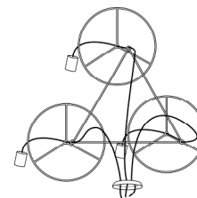
(1) Pendant Cords, Spoke Rings, Canopy & Triangle Assembly
