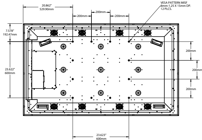
mounting diagram
