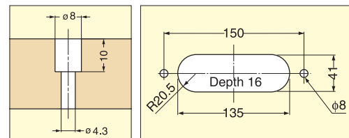
Bore Dimensions
