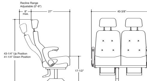
Model 2006 Recliner
