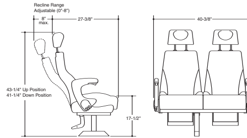
Model 2000 Recliner
