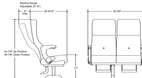
Model 2005 Recliner
