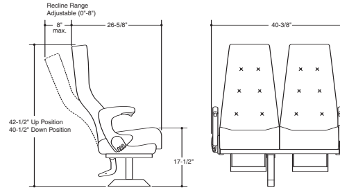
Model 2003 Recliner
