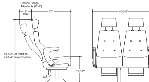
Model 2004 Recliner
