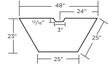
TOP SHELF FOR 96"W TRAPEZOID COMPUTER TABLE
