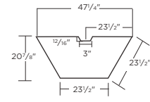
TOP SHELF FOR 80"W TRAPEZOID COMPUTER TABLE
