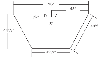
96"W TRAPEZOID COMPUTER TABLE
