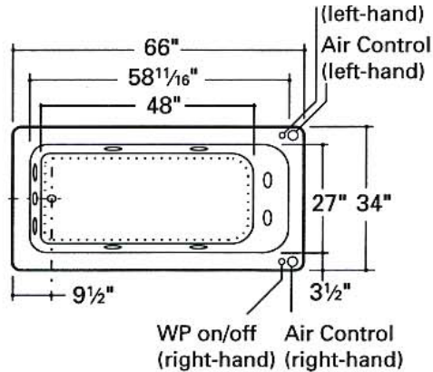
BATHTUB WITH AIR AND WHIRLPOOL CLAW 202 (left-hand) CLAW 212 (right-hand)
