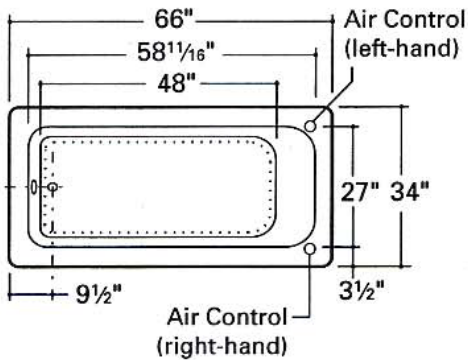
BATHTUB WITH AIR CLAT 202 (left-hand) CLAT 212 (right-hand)
