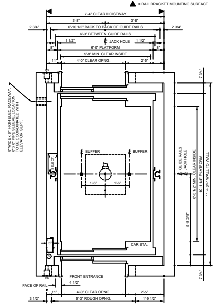
HOISTWAY PLAN NOTE: CONSULT ELEVATOR SUPP. FOR PIT SUMP LOCATION ON FRONT AND REAR ENTRANCE CASE.
