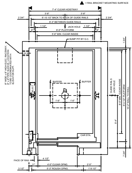
HOISTWAY PLAN
