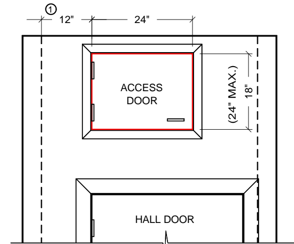
ELEVATION VIEW 'E'
