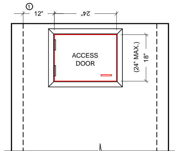
ELEVATION VIEW 'E'
