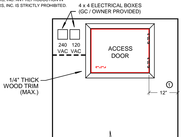
ELEVATION VIEW 'B'
