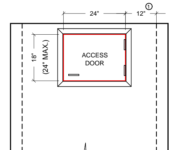
ELEVATION VIEW 'E'
