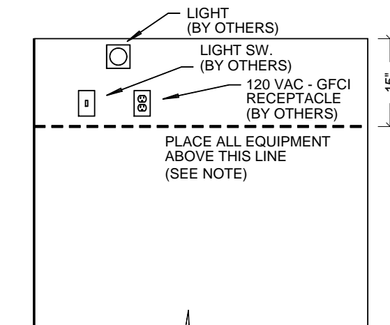
ELEVATION VIEW 'C'
