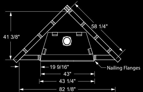
Corner Installation
