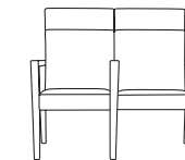
863-22H, Highback Duet with intervening arm W-49½", D-26", H-42½", SH-18¾", AH-26½"
