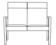
863-20H, Highback Duet W-47", D-26", H-42½", SH-18¾", AH-26½"
