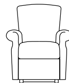
904-66, Wallsaver Recliner W=34", D=33 1/2"/66 1/2", H=40 1/4" SH=18 1/4", AH=25"
