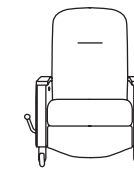
PRTT-12, Treatment Chair W=32", D=41", H=47", SH=19", AH=25"
