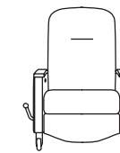
PRTT-13, Treatment Chair W=32", D=41", H=47", SH=19", AH=25"
