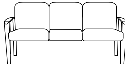
2600□-30, Three Seat W=64½", D=25", H=33½" SH=18½", AH=25½"
