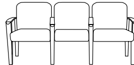
2600□-33, Three Seat with full intervening arms W=68", D=25", H=33½" SH=18½", AH=25½"
