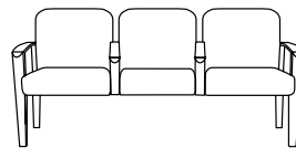
2500□-35, Three Seat with divider arms W=68", D=25", H=33¾" SH=18½", AH=25½"
