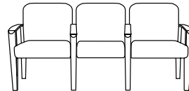
2500□-33, Three Seat with full intervening arms W=68", D=25", H=33¾" SH=18½", AH=25½"
