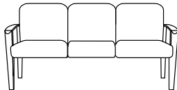
2500□-30, Three Seat W=65½", D=25", H=33¾" SH=18½", AH=25½"
