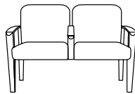
2500□-25, Two Seat with divider arm W=47", D=25", H=33¾" SH=18½", AH=25½"
