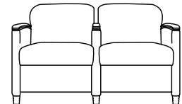
734-22, Two Seat with full intervening arm W=51½", D=27½", H=32½", SH=18", AH=23¾"
