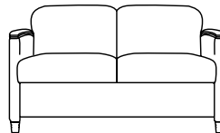
734-20, Two Seat W=49", D=27½", H=32½", SH=18", AH=23¾"
