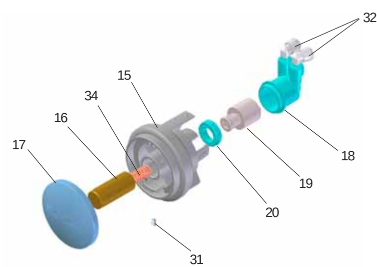
Figure 13 - Fountain Body
