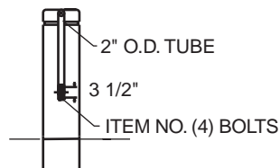
SECTION VIEW BIKE RACK
