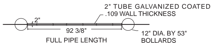
TOP VIEW BIKE RACK
