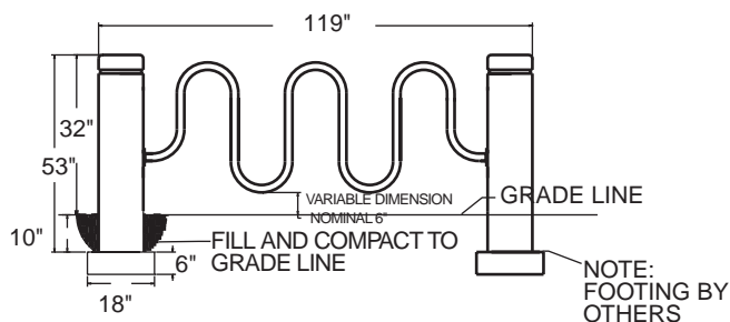
SIDE VIEW BIKE RACK
