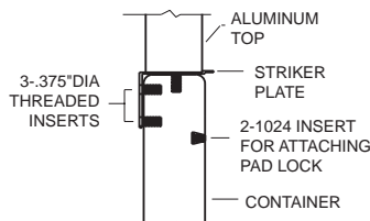
SECTION C-C NOT TO SCALE
