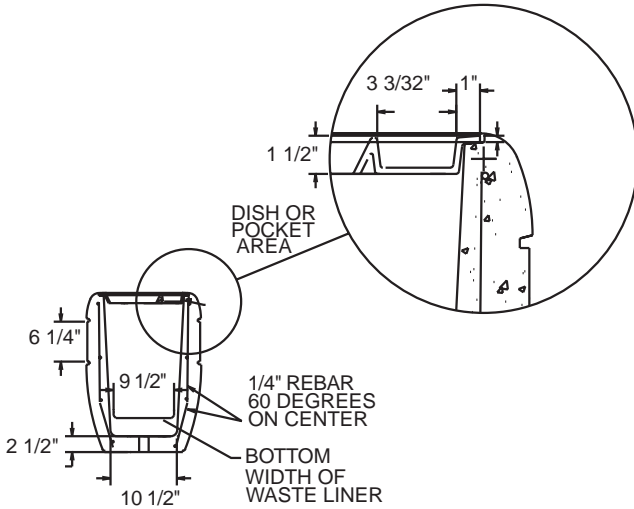
SECTION VIEW OF WASTE CONTAINER
