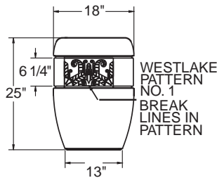
SIDE VIEW OF WASTE CONTAINER
