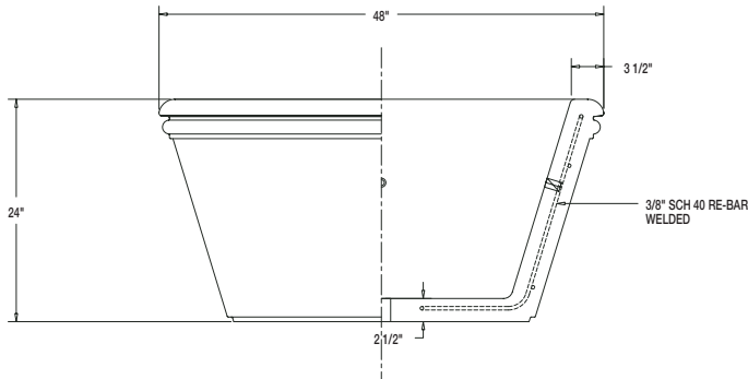
ELEVATION/SECTION VIEW PLANTER
