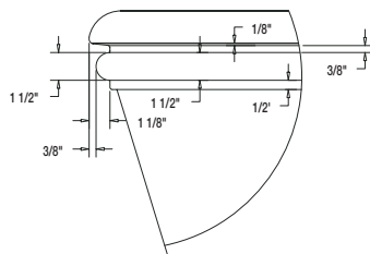
ELEVATION/SECTION VIEW PLANTER
