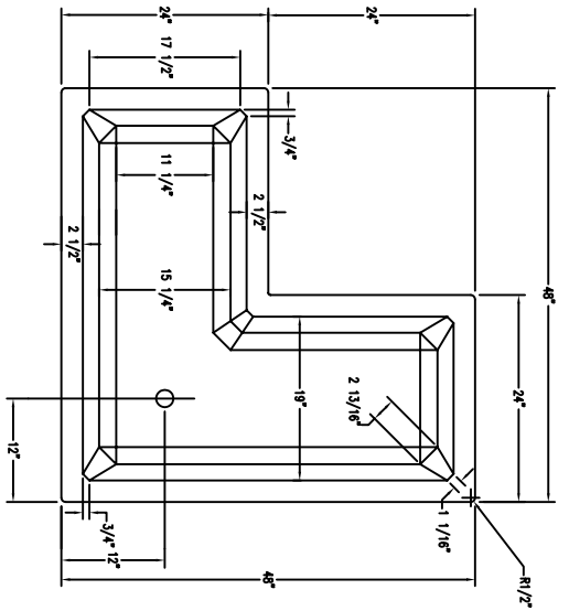
TOP VIEW CORNER PLANTER
