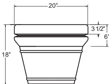
FRONT VIEW PLANTER
