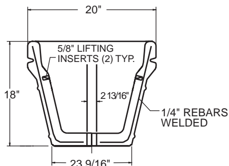
SECTION VIEW PLANTER
