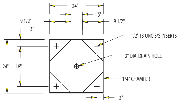
BOTTOM VIEW PLANTER
