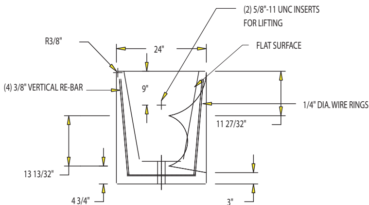
SECTION VIEW PLANTER
