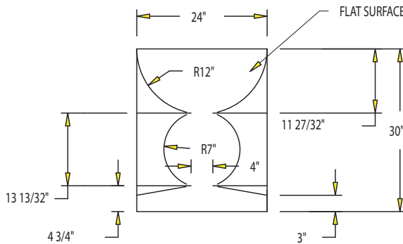
ELEVATION VIEW PLANTER
