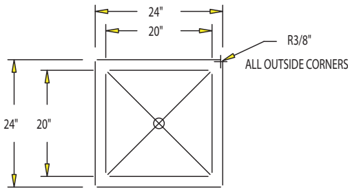
TOP VIEW PLANTER
