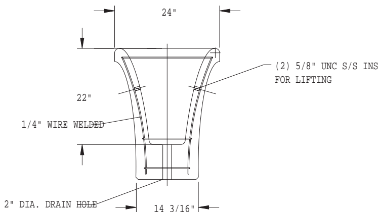
SECTION VIEW PLANTER
