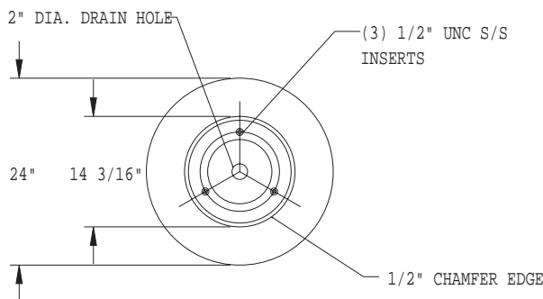
BOTTOM VIEW PLANTER
