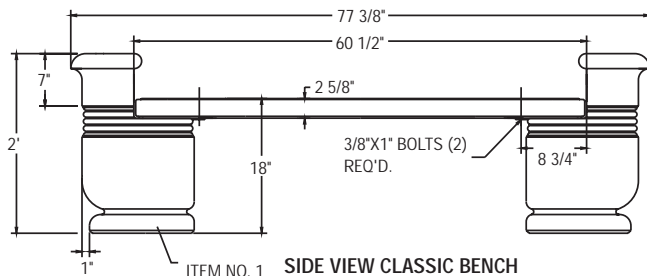
ITEM NO. 1 SIDE VIEW CLASSIC BENCH
