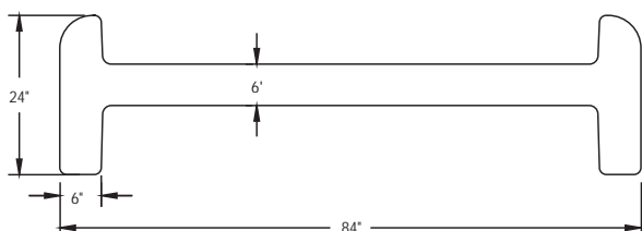
SIDE ELEVATION CAST CONCRETE BENCH
