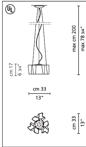
Logico micro suspension triple nested
