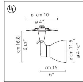
Starship wall/ceiling
