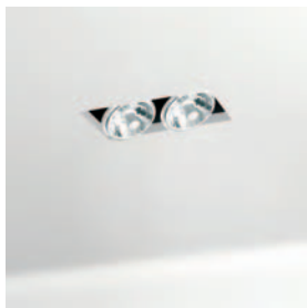
NOTHING RECTANGULAR 2 LAMPS AR111 (G53) HSR111 (GX8.5)
