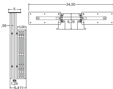
One Thin and One Thick Perforated Cover 5-3/8"W x 6-1/4"L x 4-1/2"H
