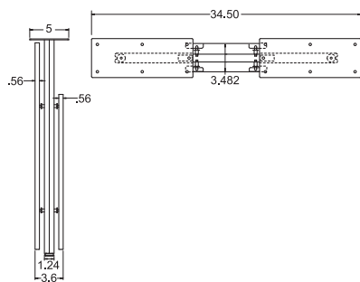
Two Thin Covers 5-3/8"W x 3-3/8"L x 4-1/2"H
