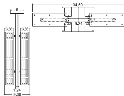
Two Thick Perforated Covers 5-3/8"W x 9"L x 4-1/2"H
