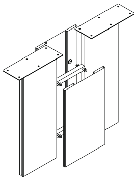
30" Metal Leg (exploded) Standard on all rectangular and arched boat tables. 30" leg consists of two 10" leg panels and a 10" metal connector plate/cover
