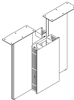
30" Metal Leg (assembly) (Assembled leg shows the removable perforated leg cover)
