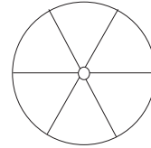
Fringe 4
