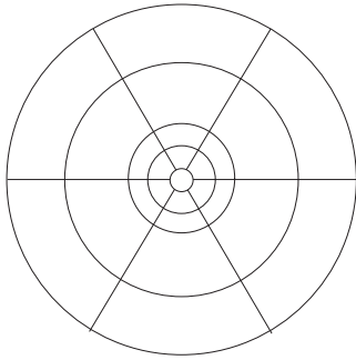
Fringe 2
