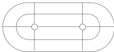
Fringe 6
