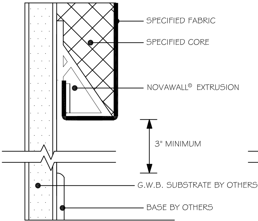
CONCEALED @ VINYL BASE
